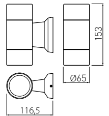
LD-BA2GU10-0M
