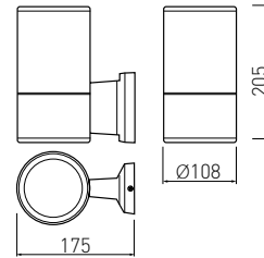
LD-BALGU10-0S
