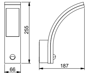
LD-PAR10W40BC-00 LD-PAR10W40BC-10
