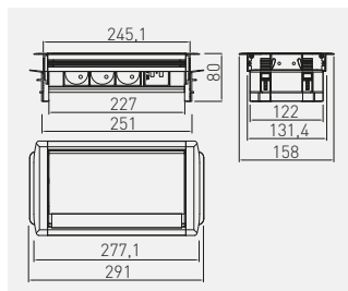
AE-PBC3GS2U-53BK
